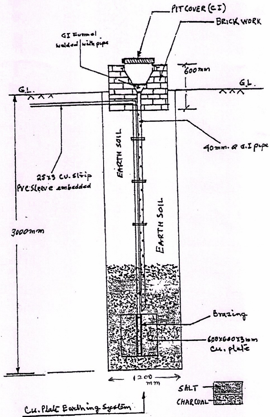
Drawing for Earthing - ①
